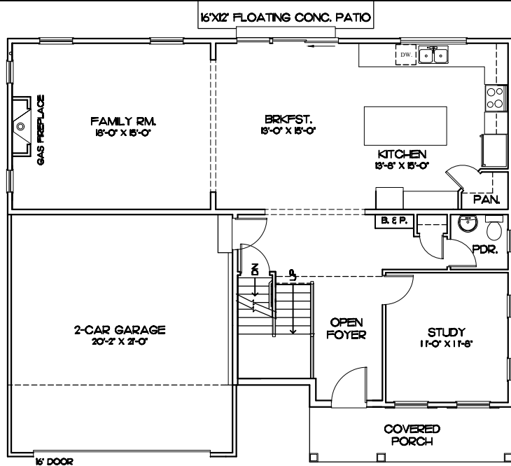
FIRST FLOOR PLAN / 9' CEILINGS
