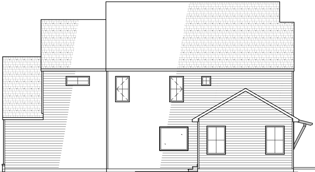
REAR ELEVATION
