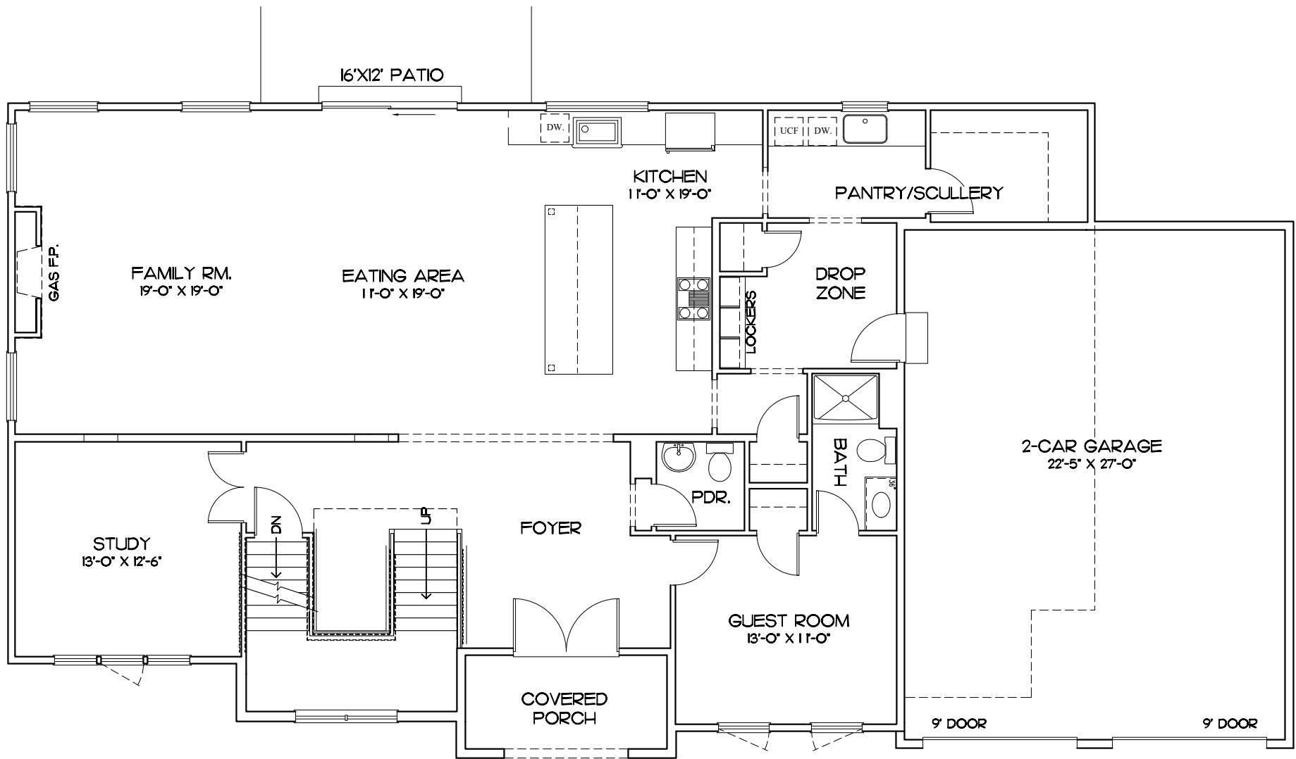
THE | Augusta Anthracite Site 2 FIRST FLOOR PLAN - 10' WALLS | 1,940 S.F.
