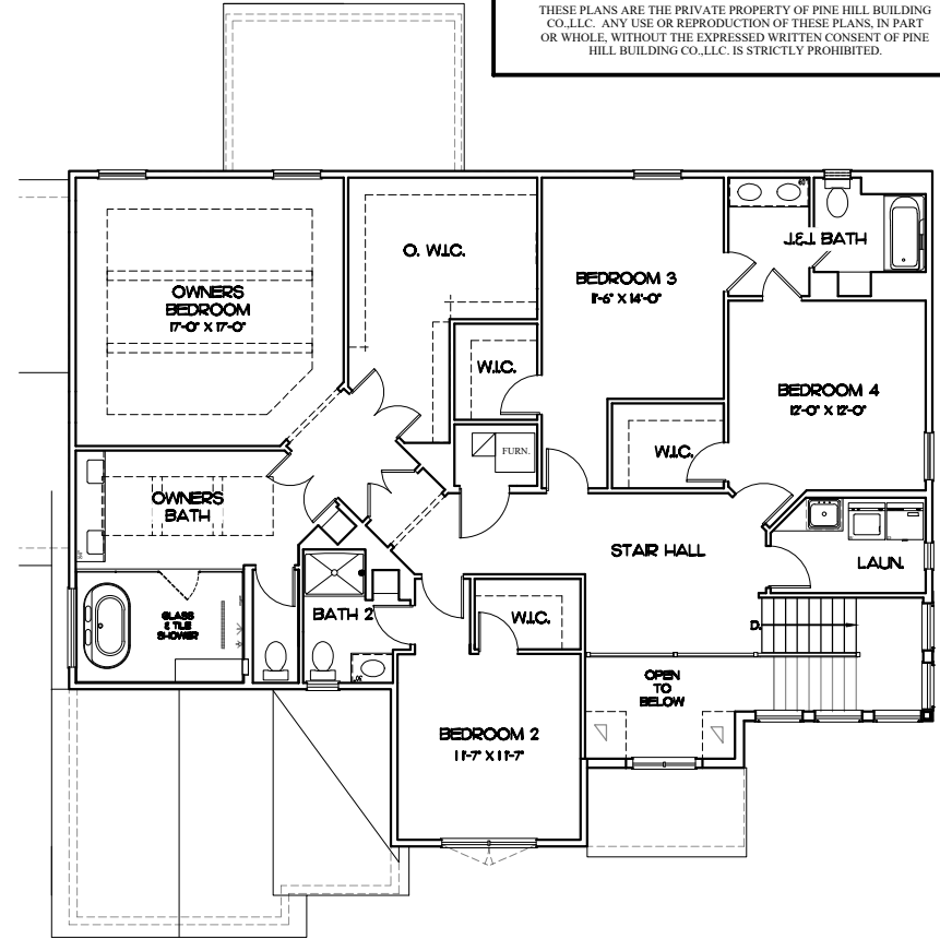
SECOND FLOOR PLAN / 9' CEILINGS
