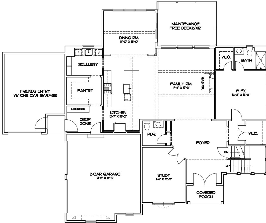
FIRST FLOOR PLAN / 10' CEILINGS
